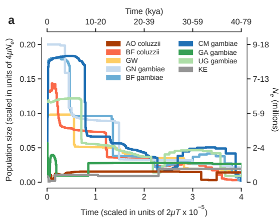
Figure a: Stairway Plot
