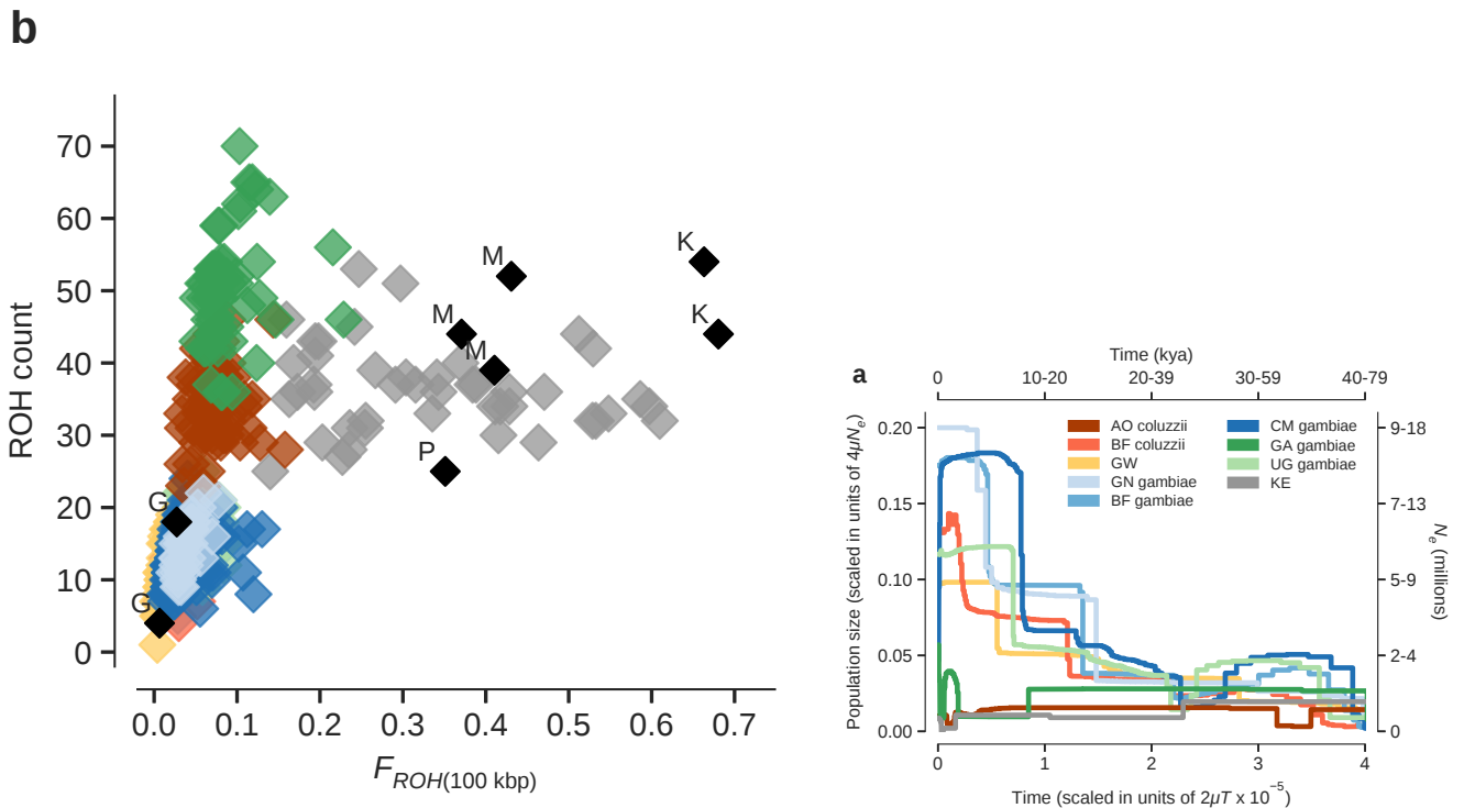
a , Stairway plot of changes in population size over time. Absolute values of time and N_e are shown on alternative axes as a range of values, assuming lower and upper limits for the mutation rate \mu as 2.8 \times 10^{-9} and 5.5 \times 10^{-9} , respectively, and t = 11 generations per year. ka, thousand years ago. b , Runs of homozygosity (ROH) in individual mosquitoes, highlighting recent inbreeding in Kenyan (grey) and colony (black) mosquitoes. G, Ghana; K, Kisumu; M, Mali; P, Pimperena.
