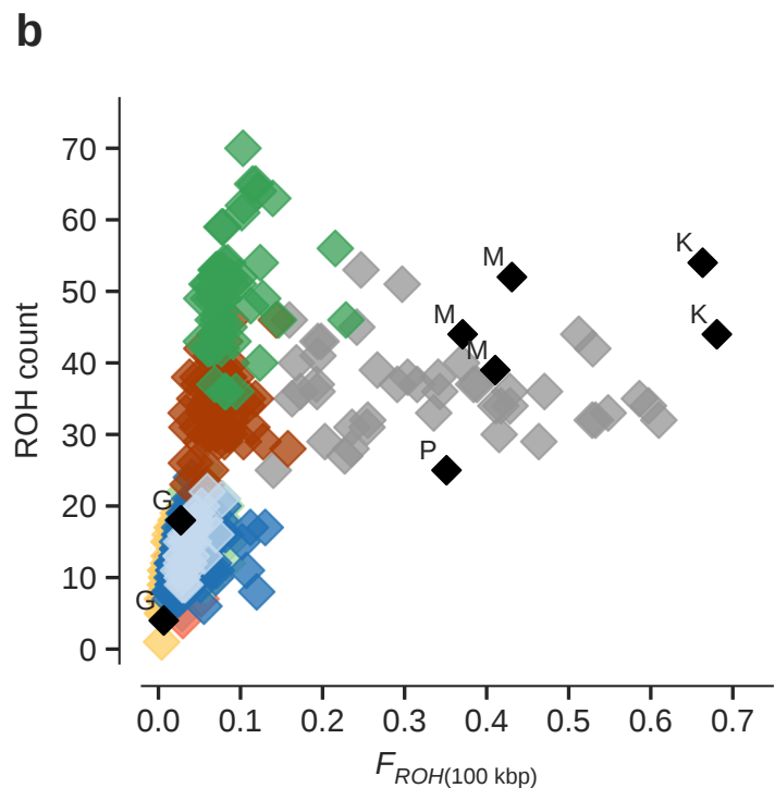
Figure b: ROH Scatter Plot
